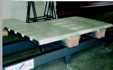
Stretch film packaging with automatic bottom feeder. No steel strap required
